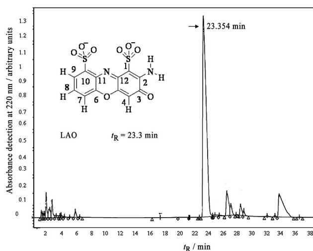
Figure 2. HPLC chromatogram of bioconversion reaction with commercial laccase Bioscreen ( Trametes versicolor ) at 25 °C with substrate 3-HOA (5 mM). pH 6 (adjusted with HCl/NaOH ), sample taken after 24 h of reaction. LAO, major red compound of interest. Elution conditions from Table 2.
