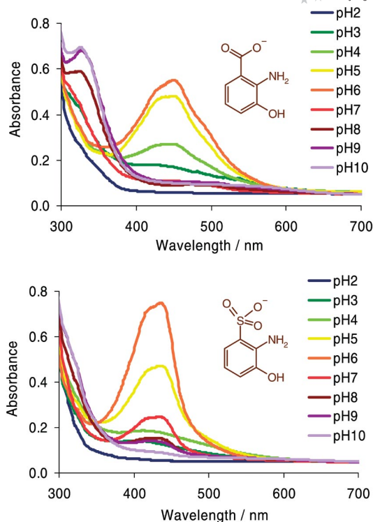
Figure 1. UV/Vis spectra of 3-HAA and 3-HOA oxidation media. Reaction media contained substrate (1 mM), laccase (100 U L -1 ) and phosphate (100 mM) at pH values ranging from 2 to 10. After 24 h incubation at 25 °C, the spectra of 10-fold diluted solutions were recorded.
