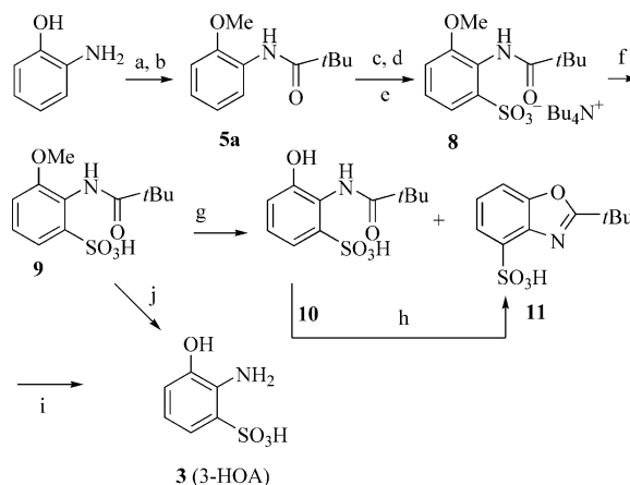
Scheme 3. Optimised synthesis of 3-hydroxyorthanilic acid.
