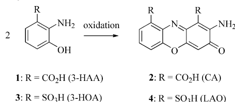
Scheme 1. Biomimetic synthesis of phenoxazinone dyes.
