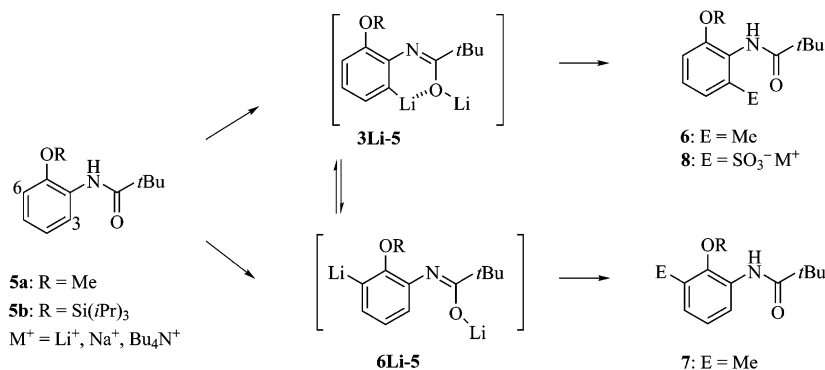
Scheme 2. Direct sulfonation: quenching of the dianion intermediate. Reagents and conditions: a) 1.1 equiv. t BuCOCl, 3 equiv. NaHCO 3 , H 2 O/EtOAc, 25\text{ }^{\circ}\text{C} 4 h; b) 1.1 equiv. MeI, 1.1 equiv. K 2 CO 3 , DMF, 0\text{ }^{\circ}\text{C} , 1 h then 25\text{ }^{\circ}\text{C} , 8 h; c) 2.4 equiv. n BuLi, THF, 0\text{ }^{\circ}\text{C} , 10 min, then 25\text{ }^{\circ}\text{C} , 3 h; d) 1.5 equiv. C 3 H 9 N·SO 3 , -10\text{ }^{\circ}\text{C} to 0\text{ }^{\circ}\text{C} , 2 h, then 25\text{ }^{\circ}\text{C} , 15 h; e) 0.9 equiv. HSO 4 ·N(Bu) 4 ; f) anion-exchange resin IRA-900, MeOH/H 2 O, then HCl/H 2 O; g) 3 equiv. BCl 3 , CH 2 Cl 2 , -20\text{ }^{\circ}\text{C} , 1 h, then 25\text{ }^{\circ}\text{C} , 8 h; h) 0.5 equiv. TFA, MeOH, 80\text{ }^{\circ}\text{C} , 3 h; i) HCl (6 N), 80\text{ }^{\circ}\text{C} , 20 h; j) HBr (48% in water), 120\text{ }^{\circ}\text{C} , 17 h.
